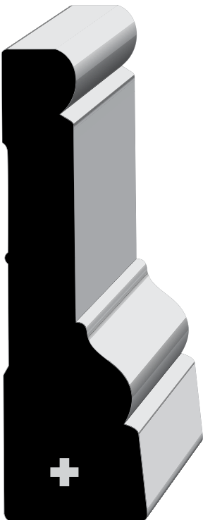
97 1-1/16" × 3-1/2"
