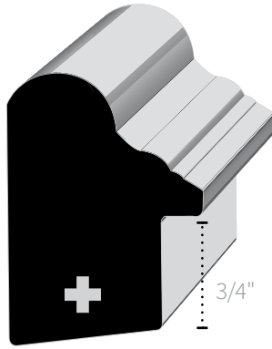
NDBB1 1-1/8" × 1-9/16"
