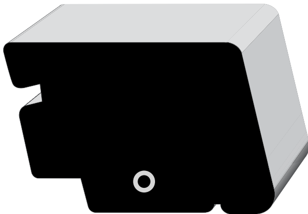
PVC7435 1-3/4" × 2-3/4"
