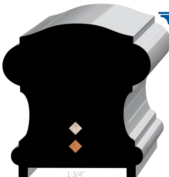
6710-PLOW 2-5/8" × 2-3/4"
