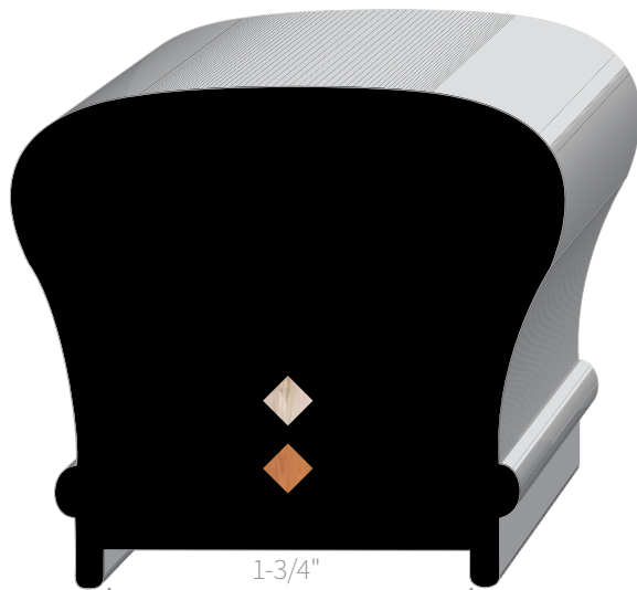
6210-PLOW 2-5/8" × 2-3/8"
